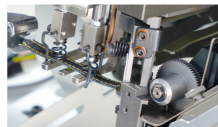
通过调整在斜切和直切模式之间转换 The conversion of angled cutting and straight cutting modes
